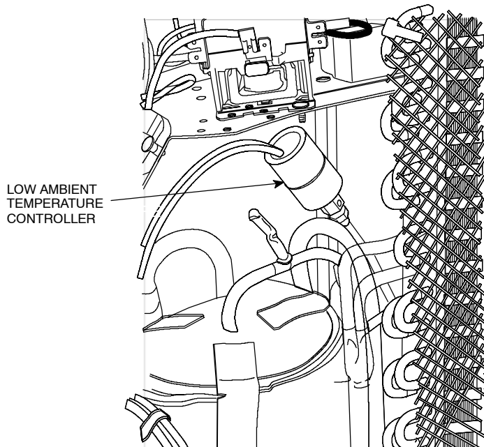
Fig. 2 – Low Ambient Temperature Control Location 38BNC/BNQ009-036
