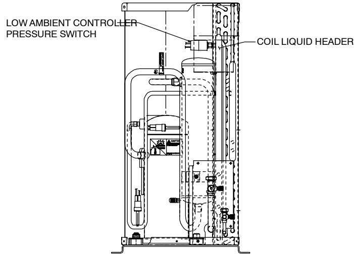
Fig. 1 – Low Ambient Control for 38HDF, HDR / 38QRF, QRR, 538A, 538E / 538B, 538Q
