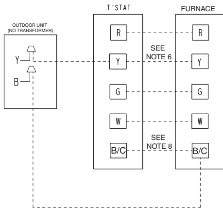
INTER-COMPONENT WIRING
