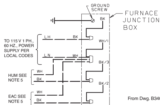
INTER-COMPONENT WIRING
