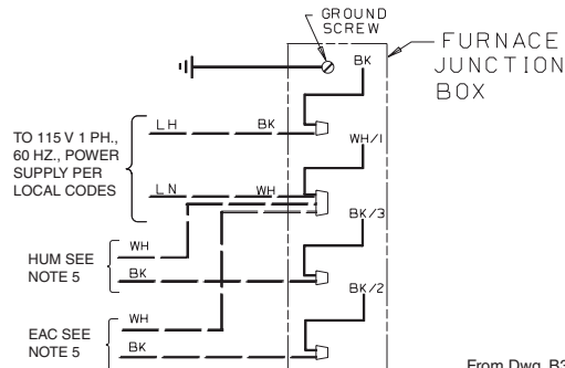
INTER-COMPONENT WIRING
