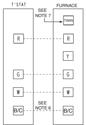
INTER-COMPONENT WIRING
