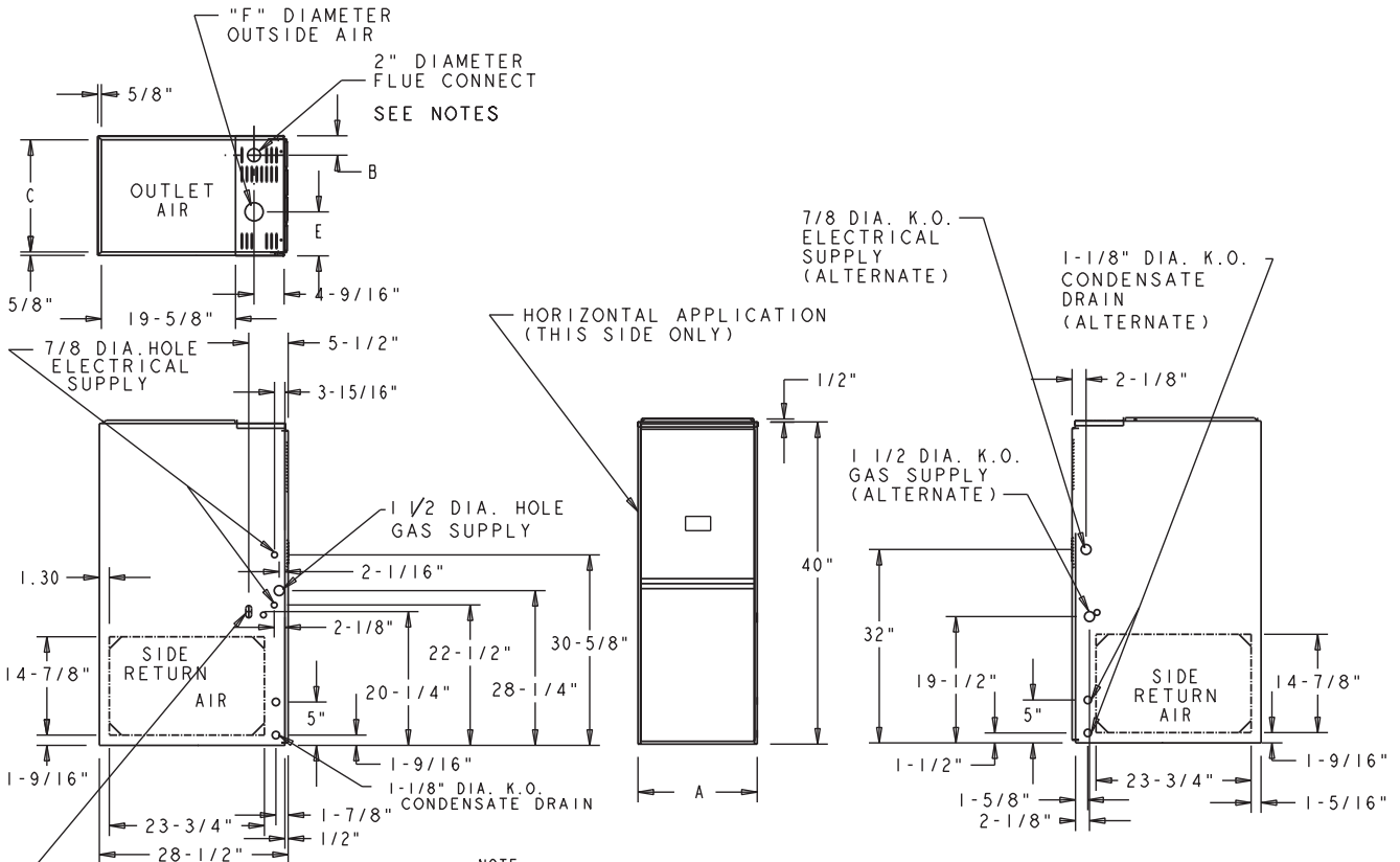
TUX-C-D Outline Drawing (ALL DIMENSIONS ARE IN INCHES)
